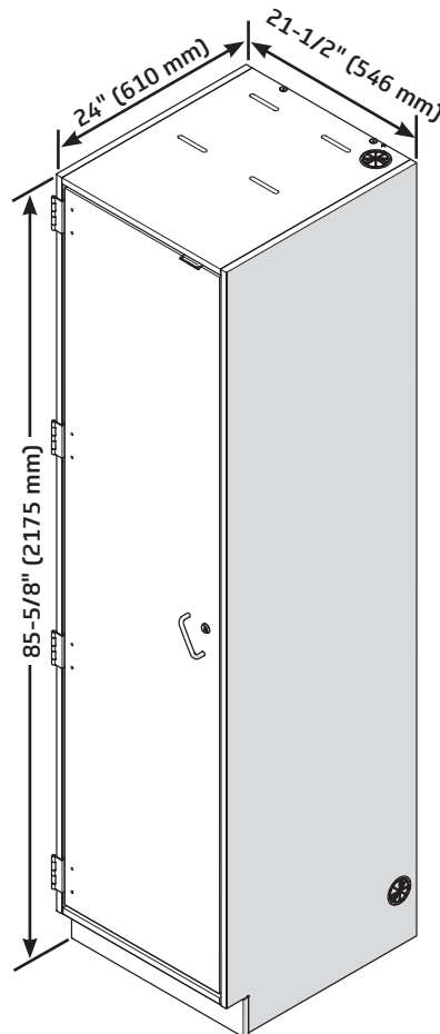
1-Column Fixed Media Storage Cabinet
