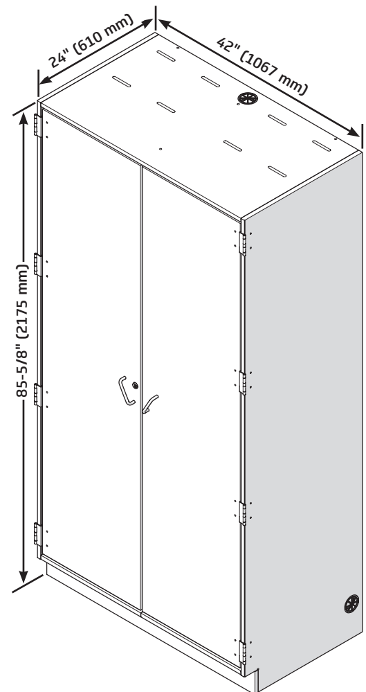
2-Column Fixed Media Storage Cabinet
